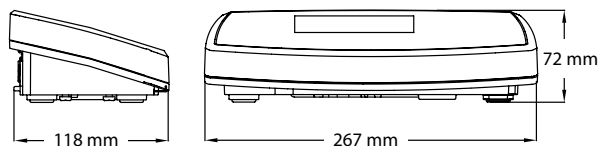
Display Dimensions for all Models
